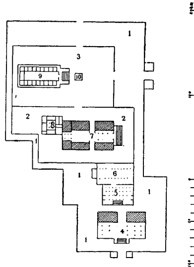
FIG. 1.—PLAN OF ROYAL BUILDINGS.
